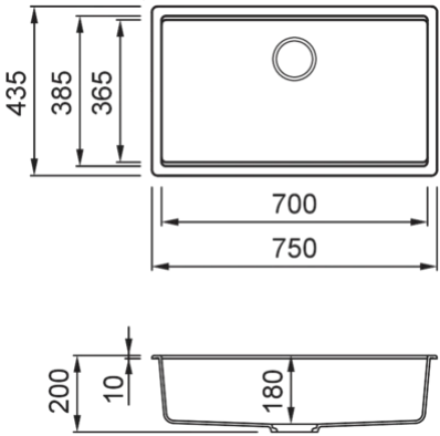
Technical Drawing
