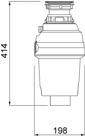
Technical Drawing
