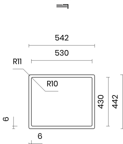
FILOTOP Flushmount
