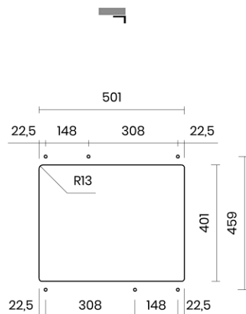
SOTTOTOP Undermount
