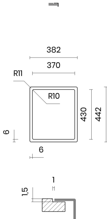
FILOTOP Flushmount
