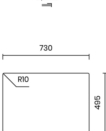
SOPRATOP Topmount
